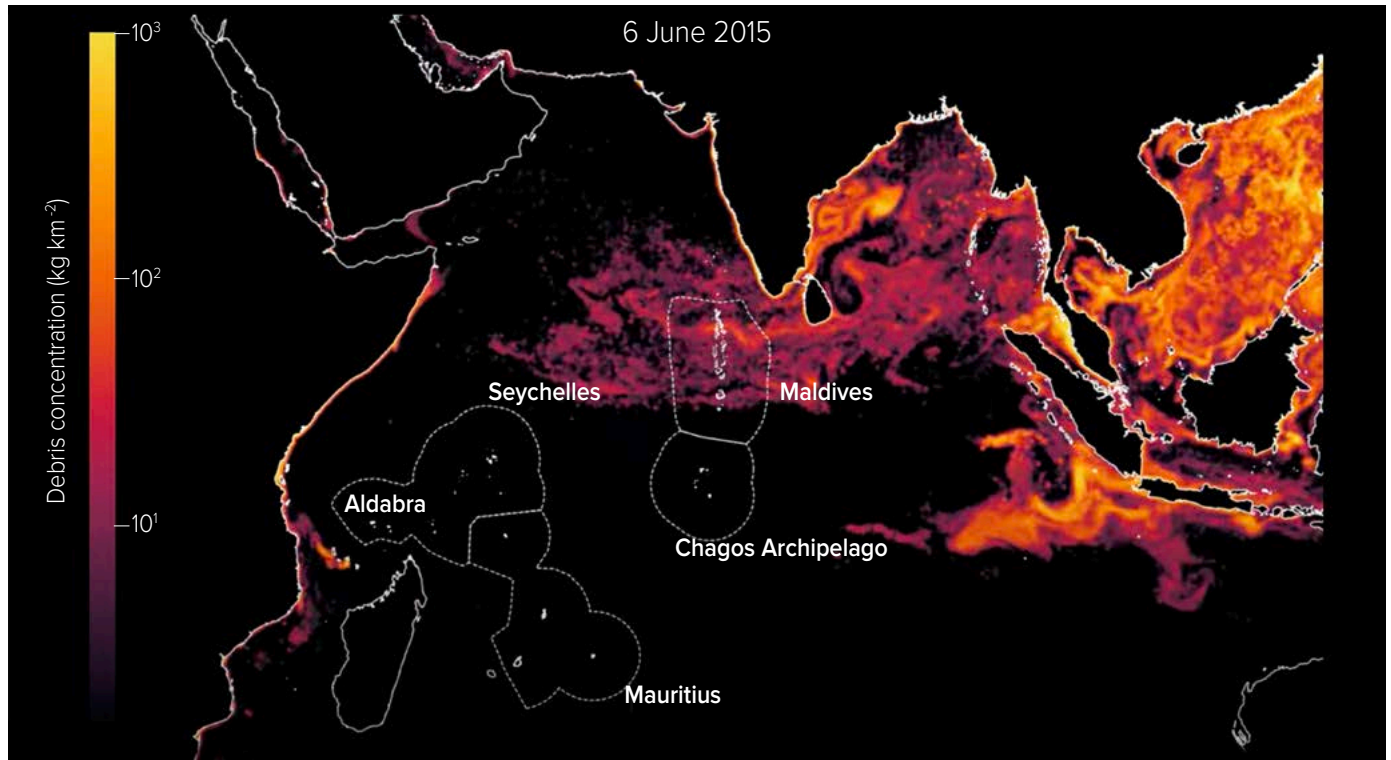
Image: Still from a video based on a numerical model developed by Vogt-Vincent et al. 2023. © Noam Vogt-Vincent 98 .
